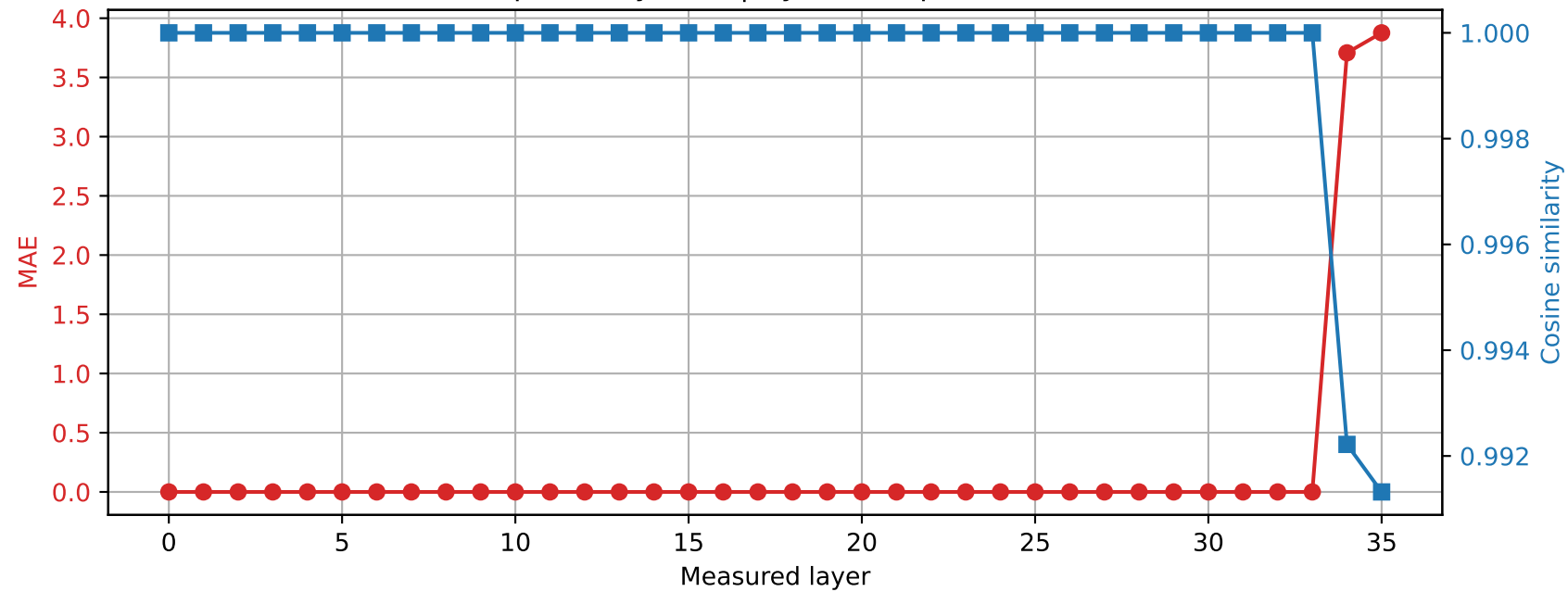
Qwen2.5-3B | Prompt 3 Spared layer 33 | Hybrid vs quantized
