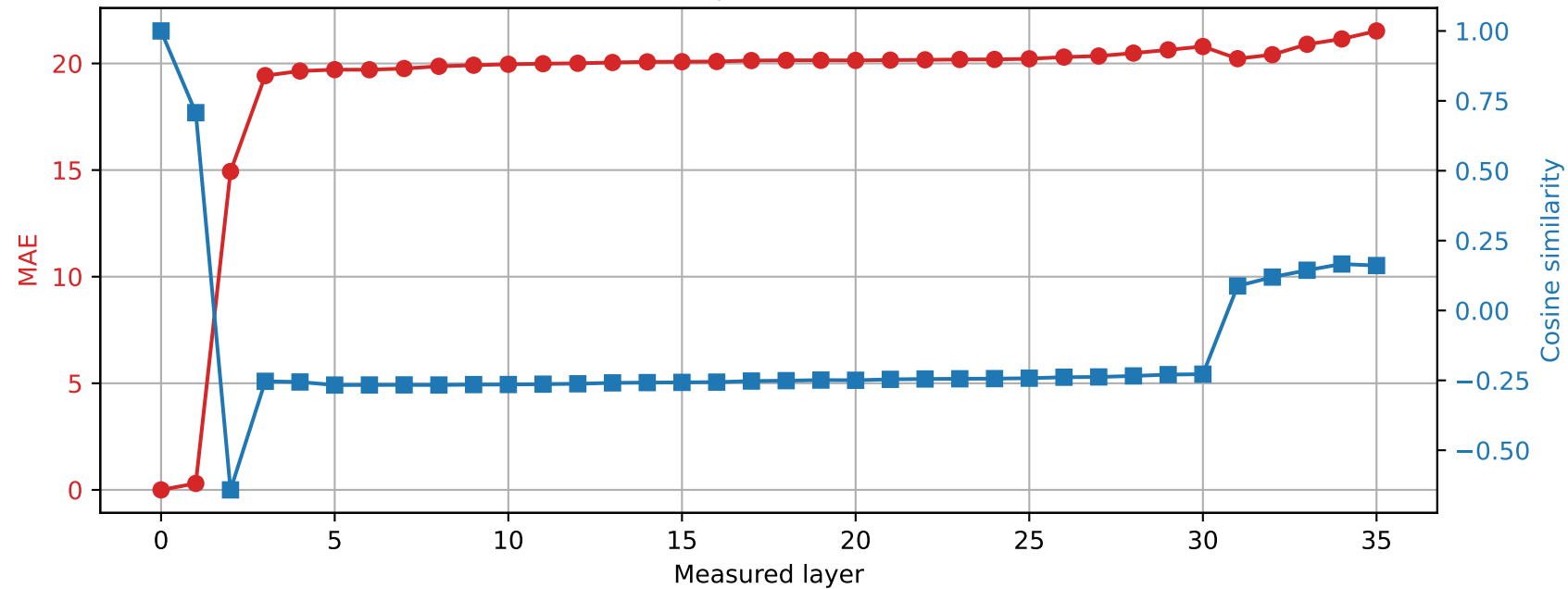
Qwen2.5-3B | Prompt 3 Spared layer 35 | Hybrid vs unquantized
