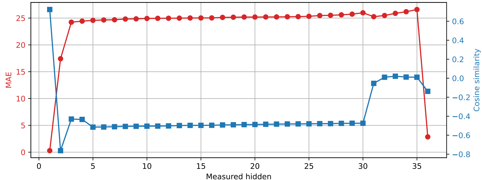
Qwen2.5-3B | Prompt 4 Spared layer 6 | Unquantized vs hybrid
