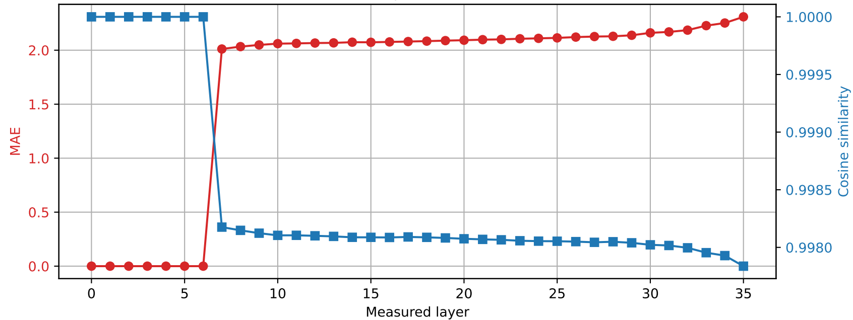
Qwen2.5-3B | Prompt 4 Spared layer 6 | Hybrid vs quantized
