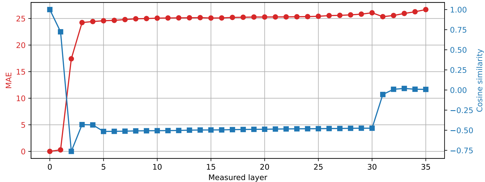
Qwen2.5-3B | Prompt 4 Spared layer 14 | Hybrid vs unquantized
