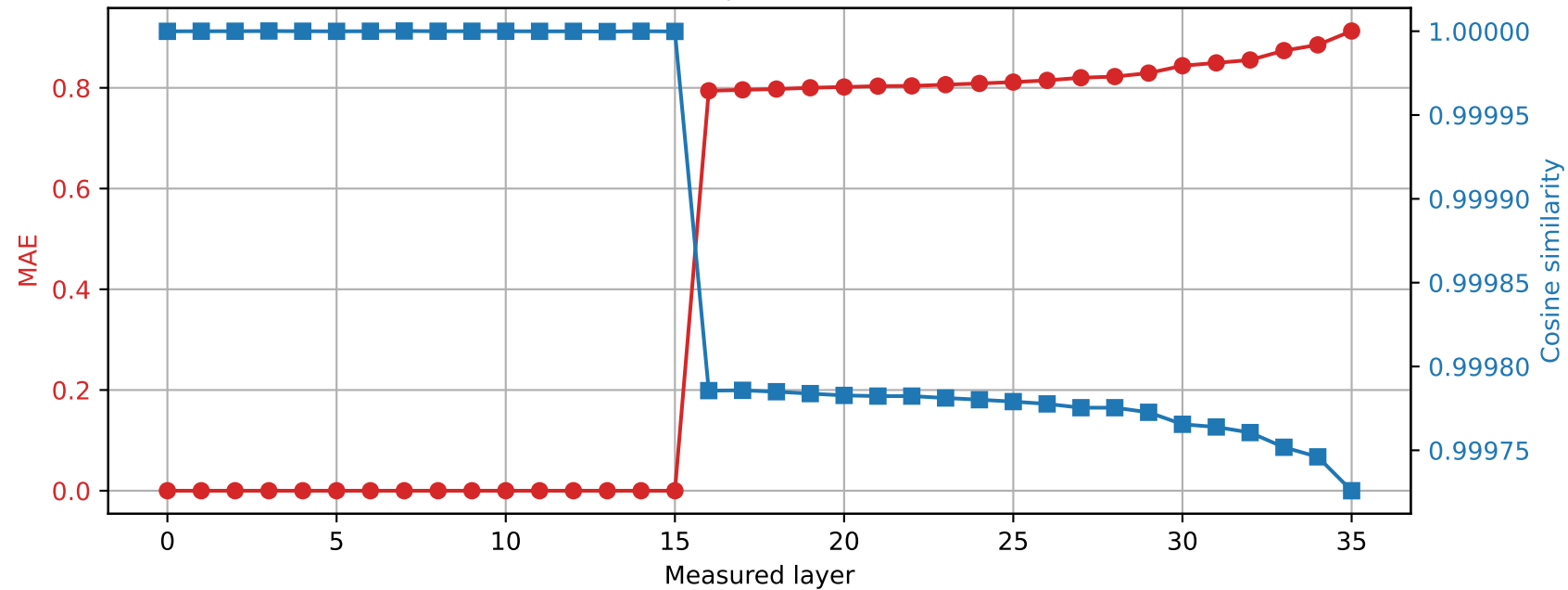
Qwen2.5-3B | Prompt 4 Spared layer 15 | Hybrid vs quantized
