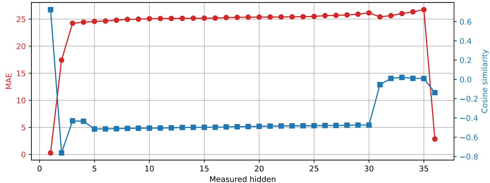
Qwen2.5-3B | Prompt 4 Spared layer 19 | Unquantized vs hybrid
