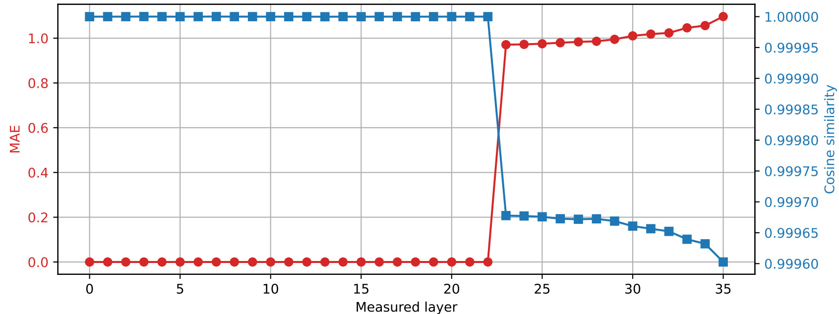
Qwen2.5-3B | Prompt 4 Spared layer 22 | Hybrid vs quantized
