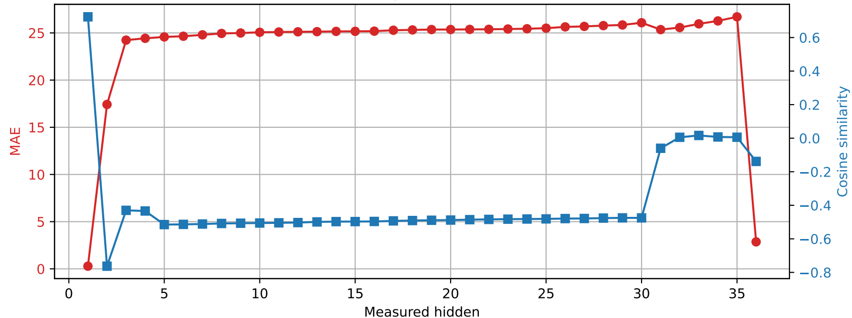
Qwen2.5-3B | Prompt 4 Spared layer 28 | Unquantized vs hybrid
