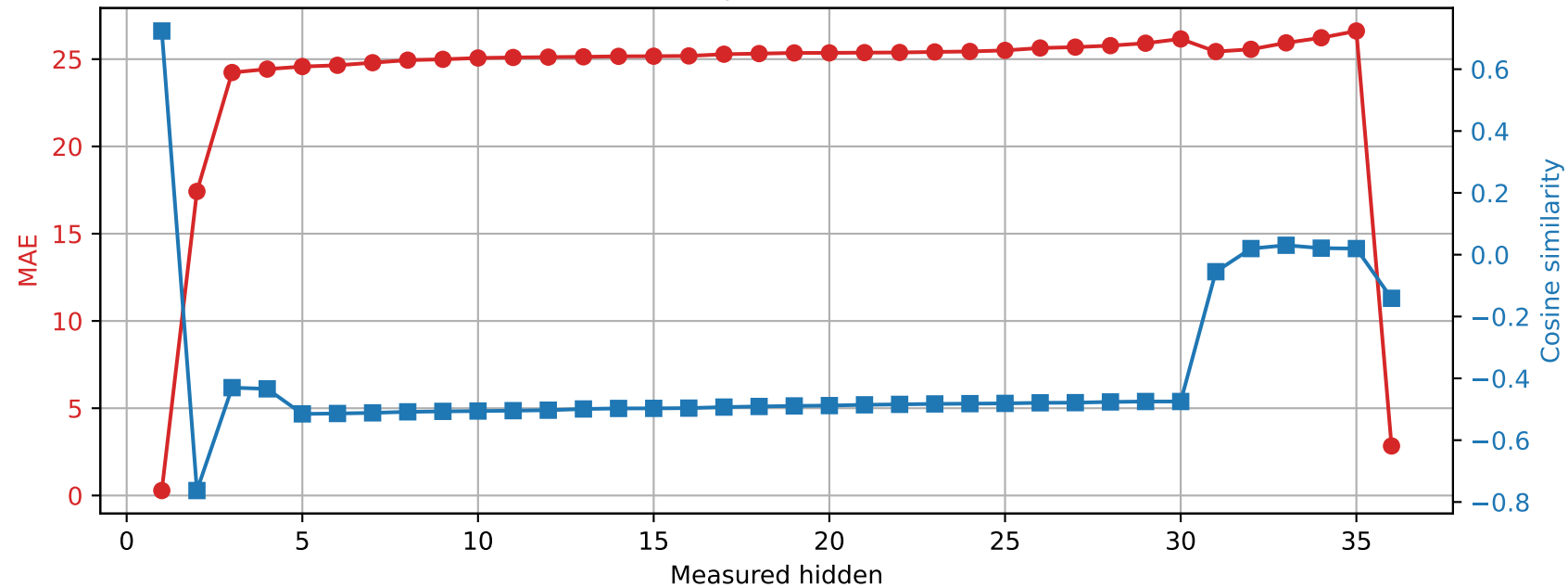
Qwen2.5-3B | Prompt 4 Spared layer 31 | Unquantized vs hybrid
