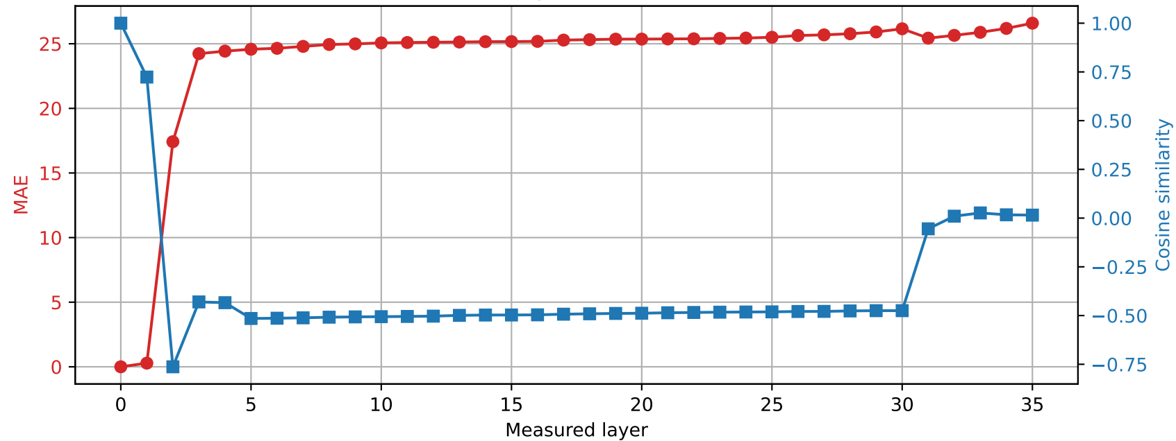
Qwen2.5-3B | Prompt 4 Spared layer 32 | Hybrid vs unquantized
