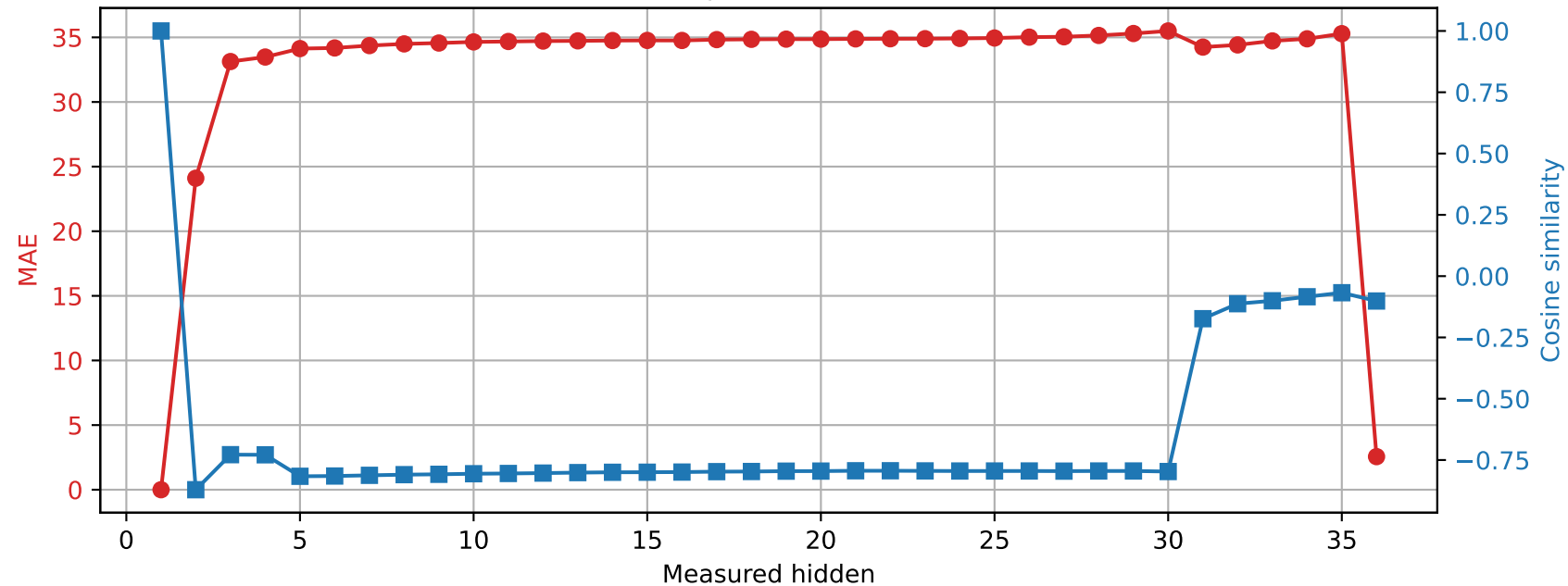
Qwen2.5-3B | Prompt 0 Spared layer 0 | Unquantized vs hybrid
