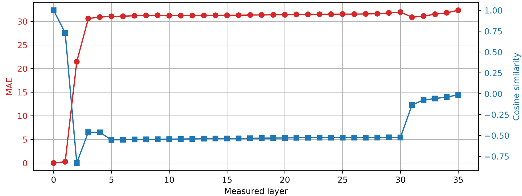
Qwen2.5-3B | Prompt 0 Spared layer 9 | Hybrid vs unquantized
