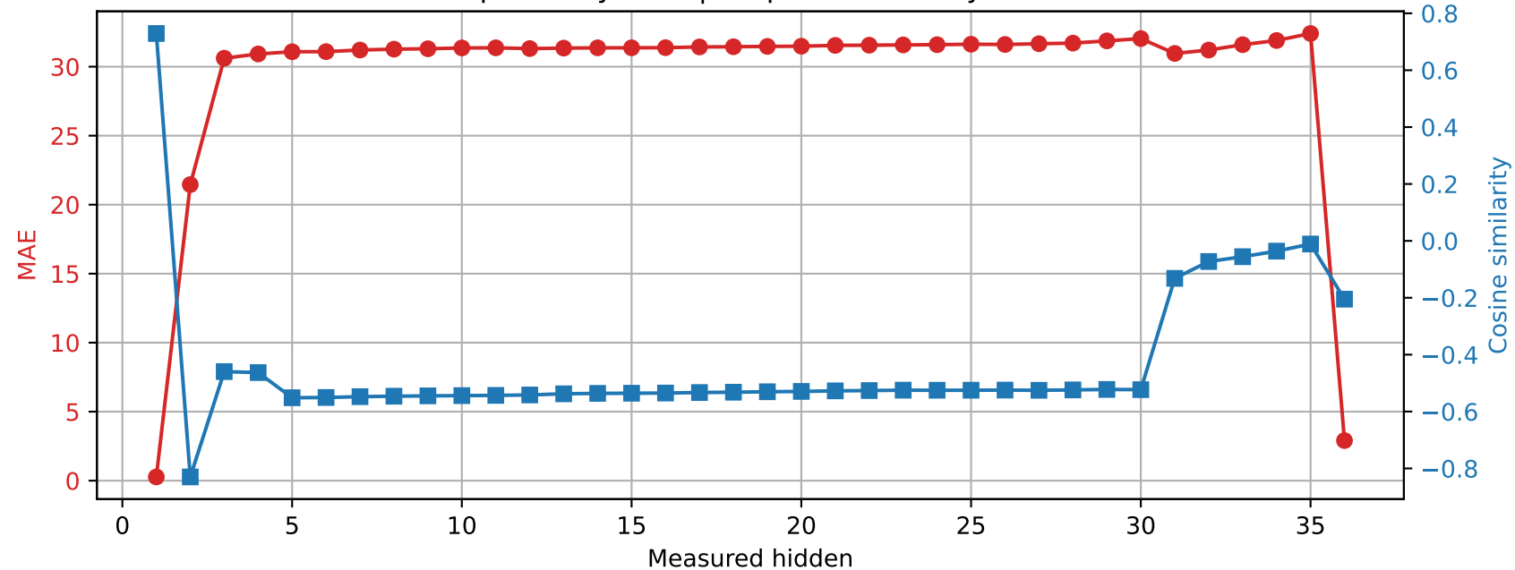
Qwen2.5-3B | Prompt 0 Spared layer 11 | Unquantized vs hybrid
