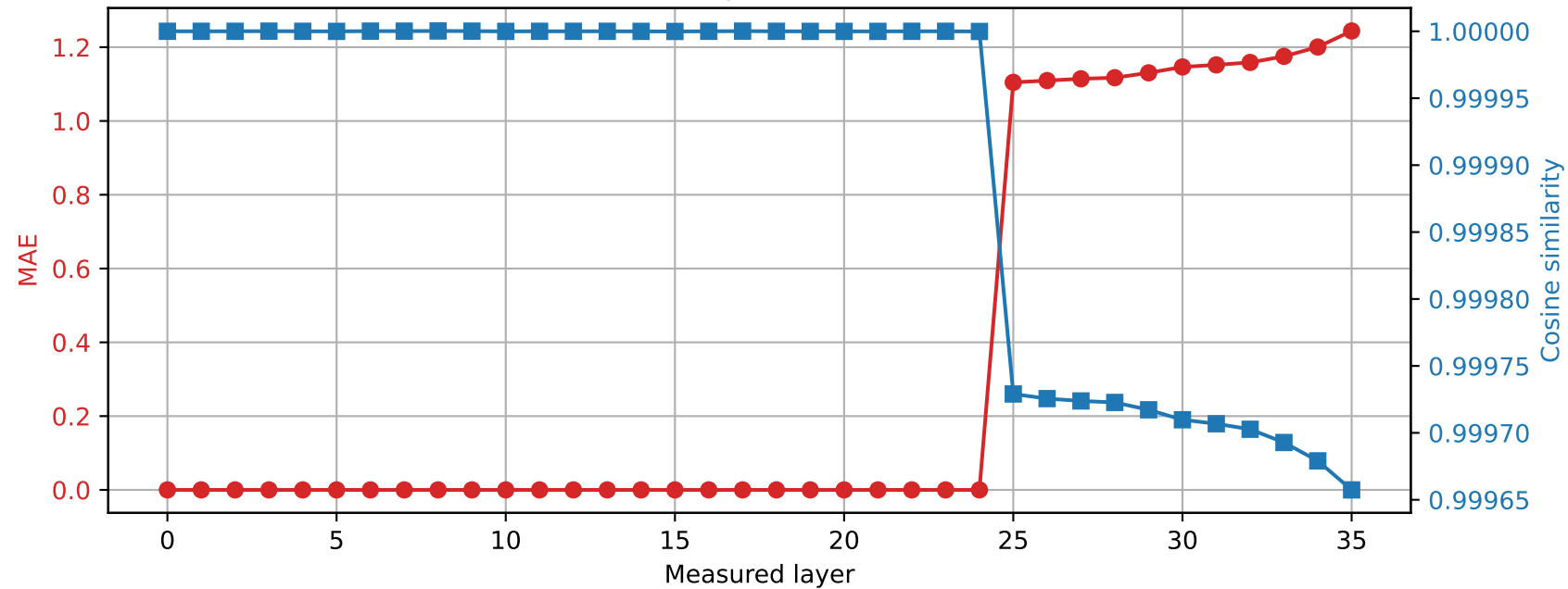
Qwen2.5-3B | Prompt 0 Spared layer 24 | Hybrid vs quantized
