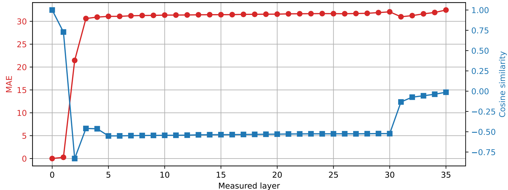
Qwen2.5-3B | Prompt 0 Spared layer 24 | Hybrid vs unquantized
