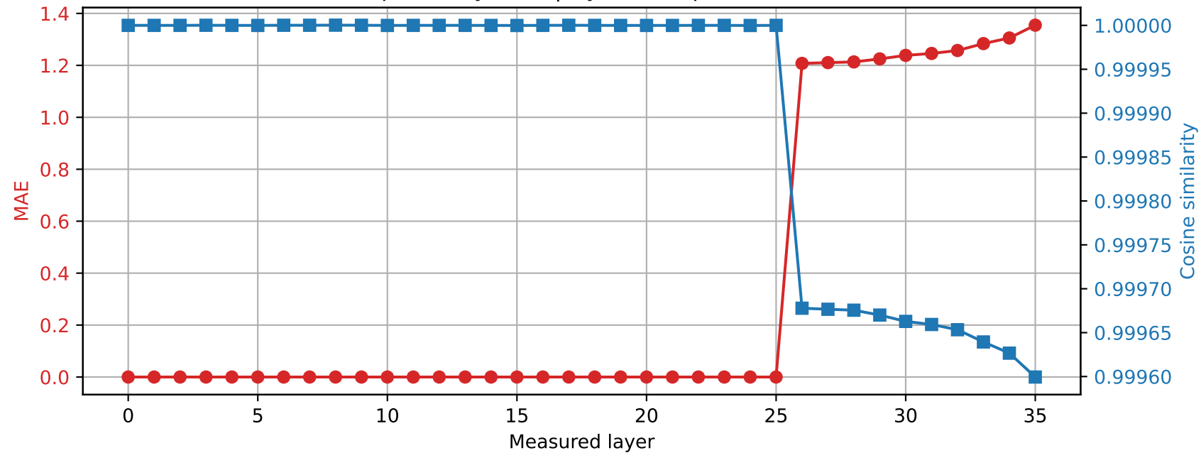
Qwen2.5-3B | Prompt 0 Spared layer 25 | Hybrid vs quantized
