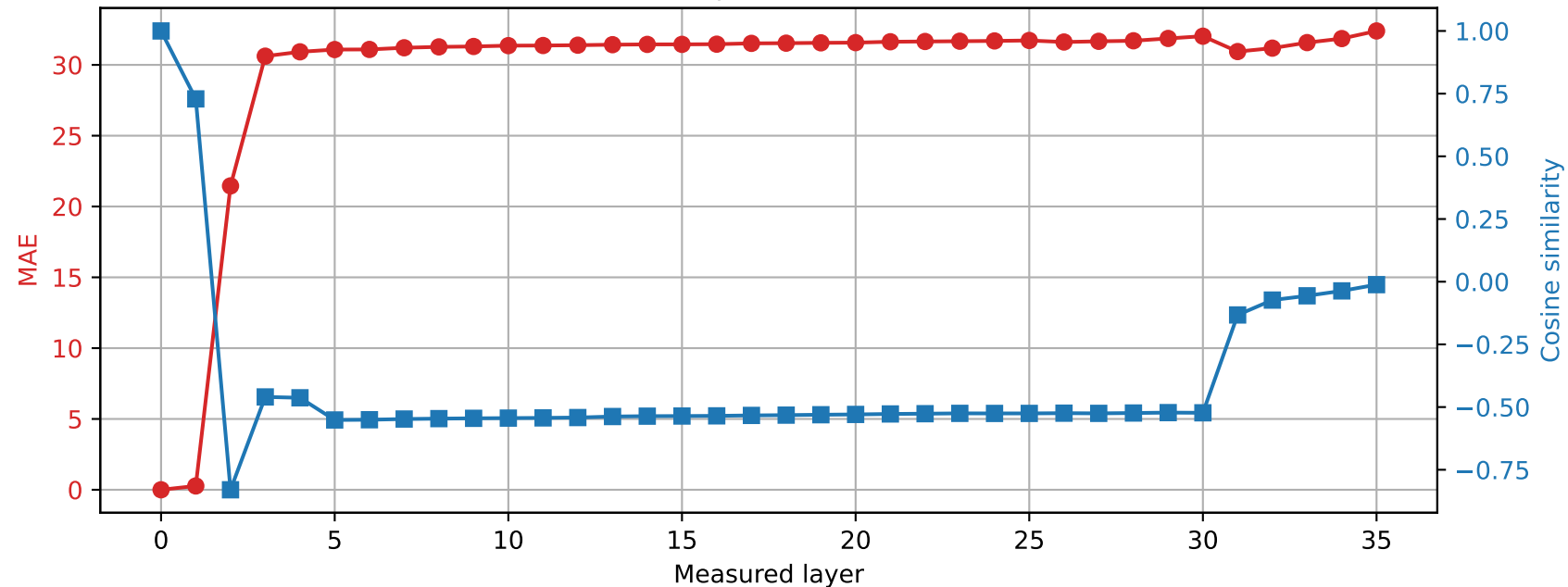
Qwen2.5-3B | Prompt 0 Spared layer 25 | Hybrid vs unquantized
