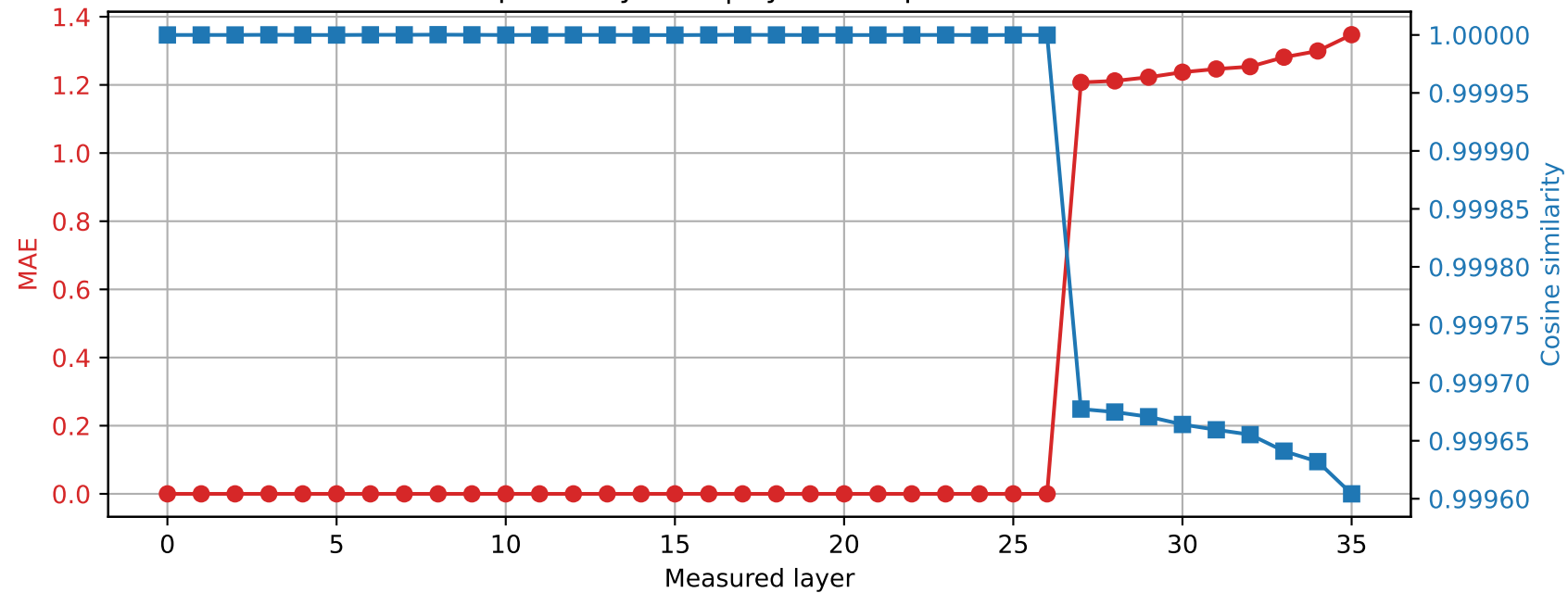
Qwen2.5-3B | Prompt 0 Spared layer 26 | Hybrid vs quantized
