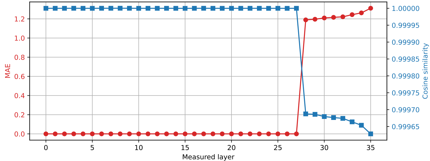
Qwen2.5-3B | Prompt 0 Spared layer 27 | Hybrid vs quantized
