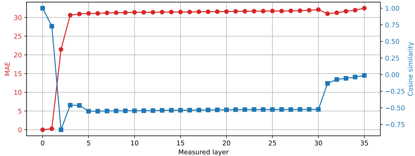
Qwen2.5-3B | Prompt 0 Spared layer 28 | Hybrid vs unquantized
