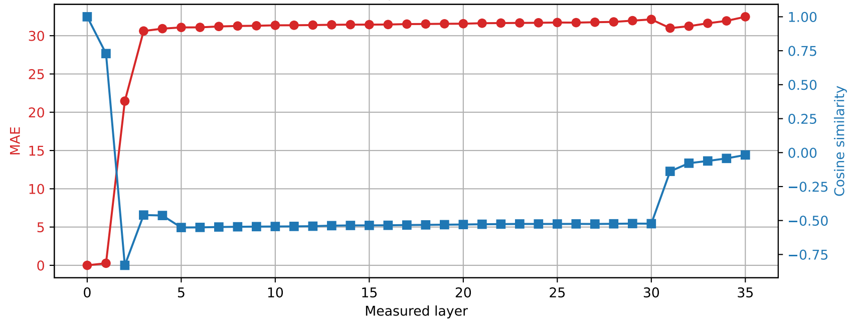
Qwen2.5-3B | Prompt 0 Spared layer 30 | Hybrid vs unquantized
