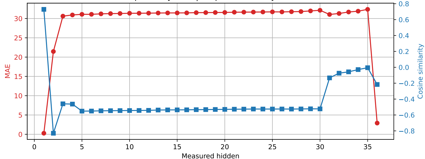
Qwen2.5-3B | Prompt 0 Spared layer 33 | Unquantized vs hybrid
