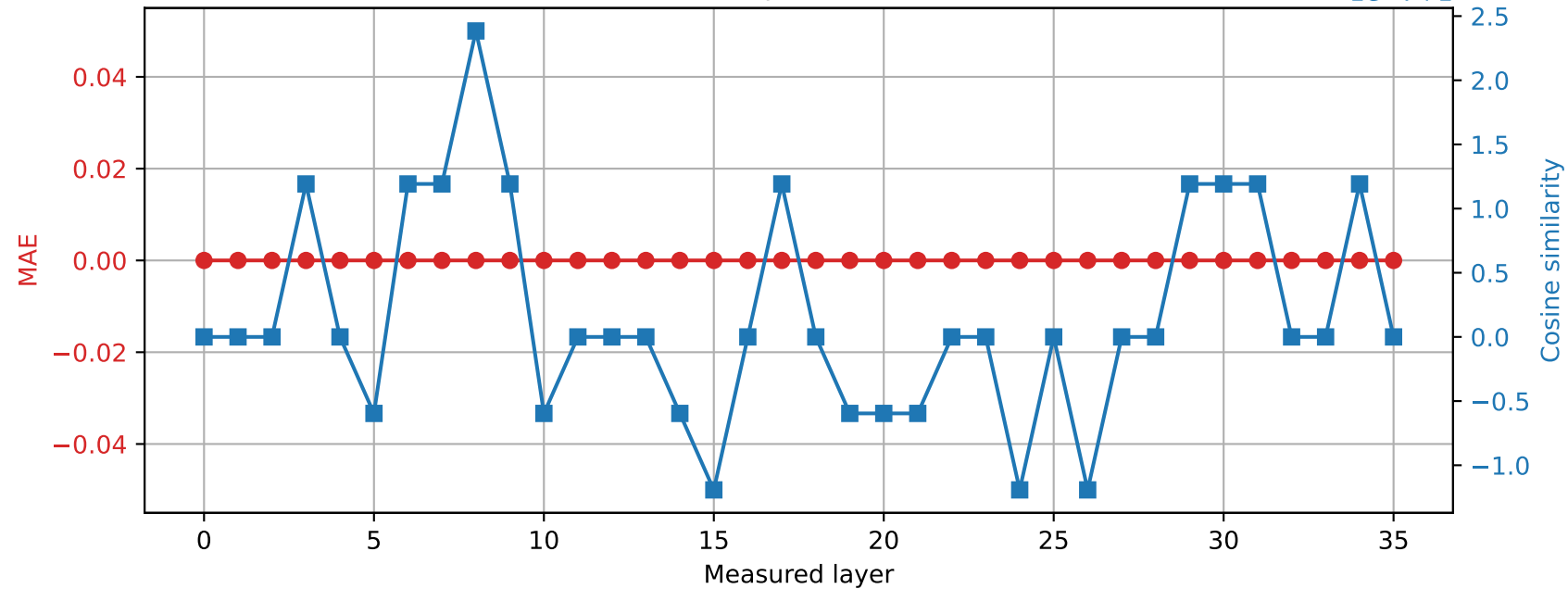
Qwen2.5-3B | Prompt 0 Spared layer 35 | Hybrid vs quantized
