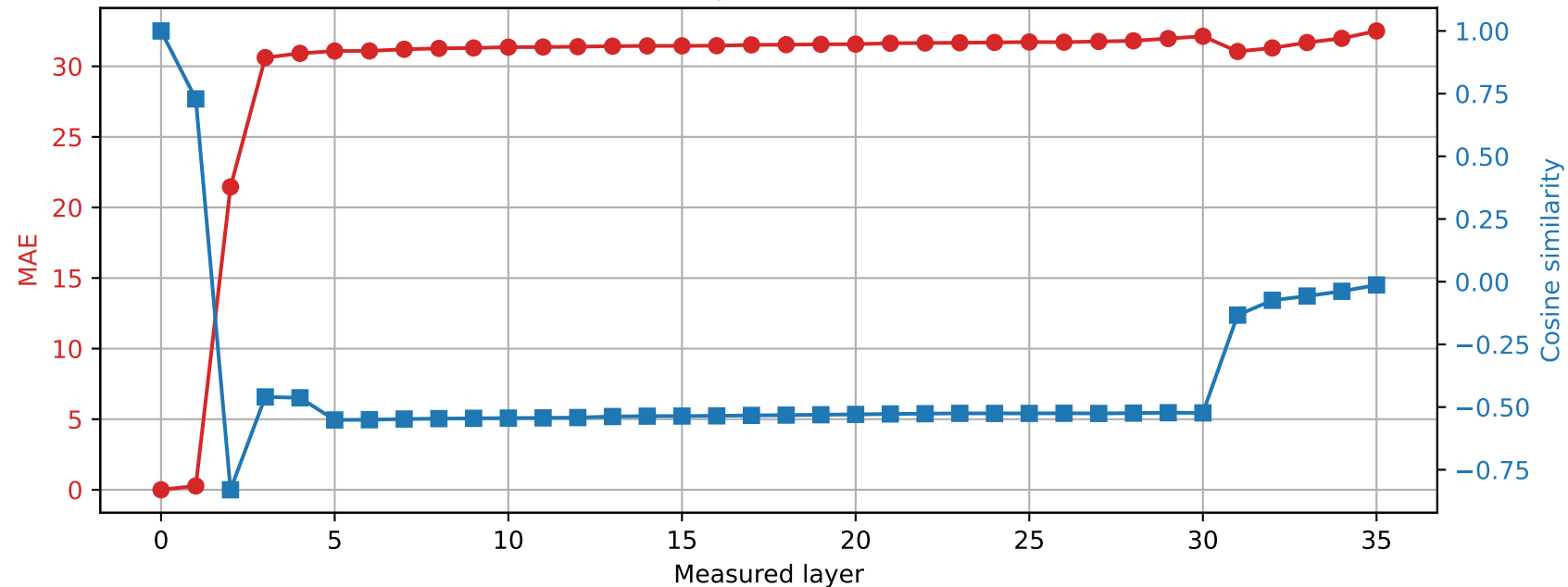
Qwen2.5-3B | Prompt 0 Spared layer 35 | Hybrid vs unquantized
