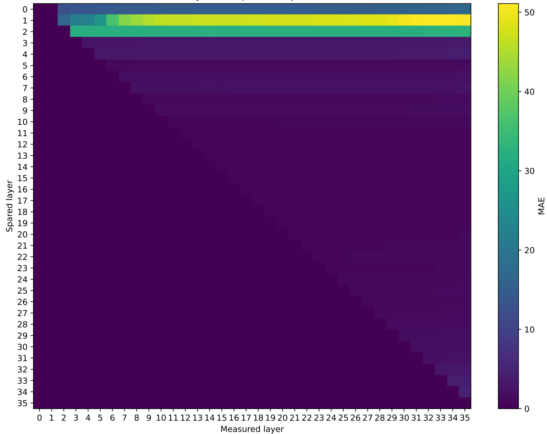
Qwen2.5-3B | Prompt 1 Hybrid vs quantized | int4
