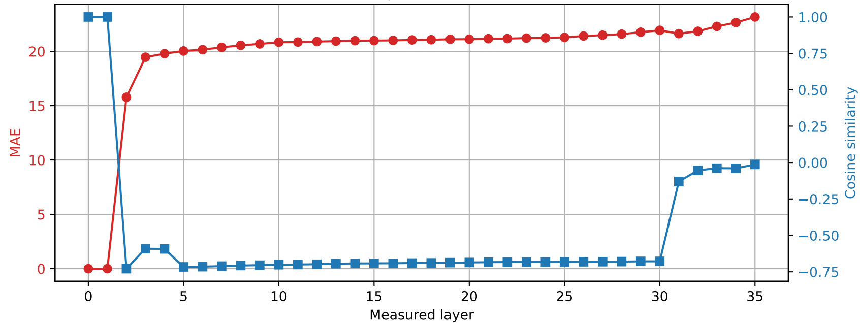
Qwen2.5-3B | Prompt 1 Spared layer 0 | Hybrid vs unquantized
