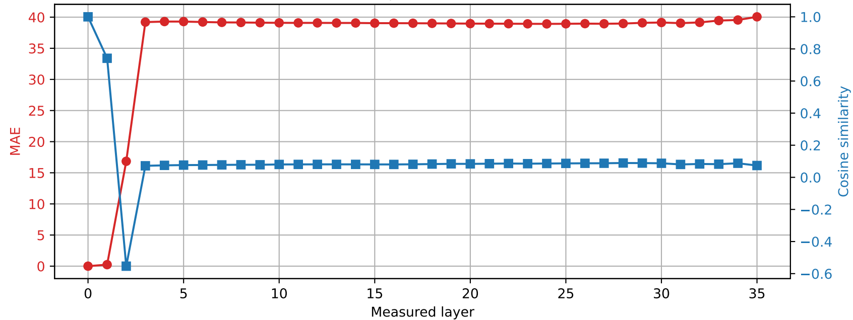
Qwen2.5-3B | Prompt 1 Spared layer 2 | Hybrid vs unquantized
