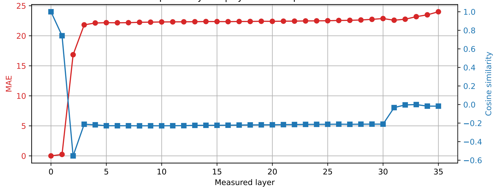
Qwen2.5-3B | Prompt 1 Spared layer 3 | Hybrid vs unquantized
