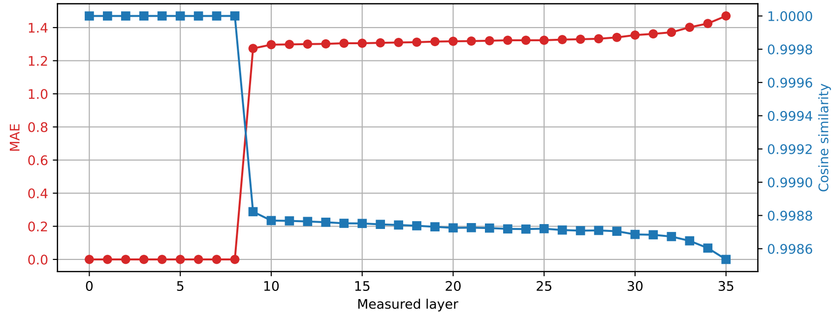
Qwen2.5-3B | Prompt 1 Spared layer 8 | Hybrid vs quantized
