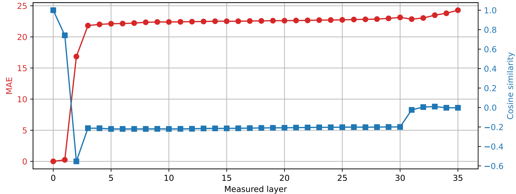
Qwen2.5-3B | Prompt 1 Spared layer 9 | Hybrid vs unquantized
