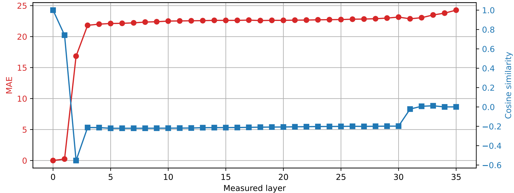
Qwen2.5-3B | Prompt 1 Spared layer 17 | Hybrid vs unquantized
