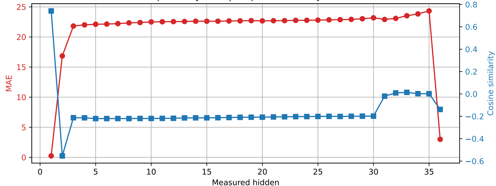
Qwen2.5-3B | Prompt 1 Spared layer 19 | Unquantized vs hybrid
