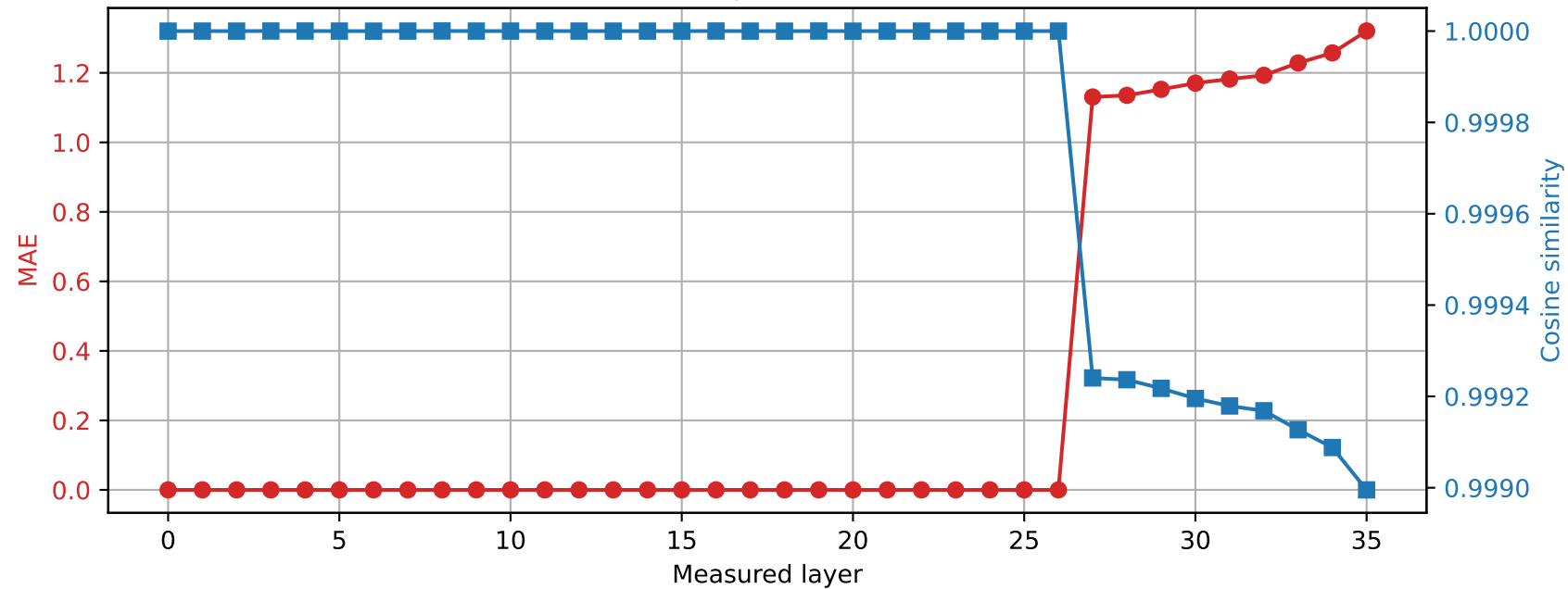
Qwen2.5-3B | Prompt 1 Spared layer 26 | Hybrid vs quantized
