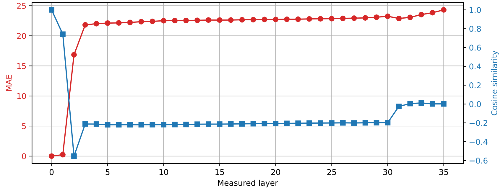
Qwen2.5-3B | Prompt 1 Spared layer 30 | Hybrid vs unquantized
