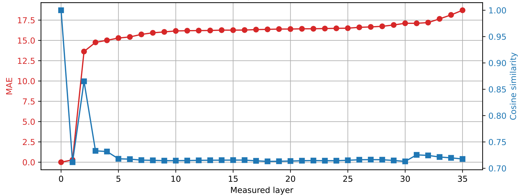
Qwen2.5-3B | Prompt 2 Spared layer 0 | Hybrid vs quantized
