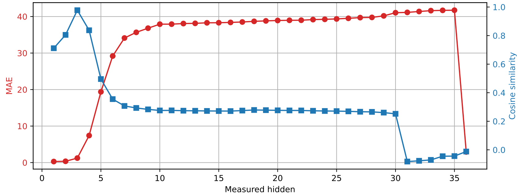
Qwen2.5-3B | Prompt 2 Spared layer 1 | Unquantized vs hybrid
