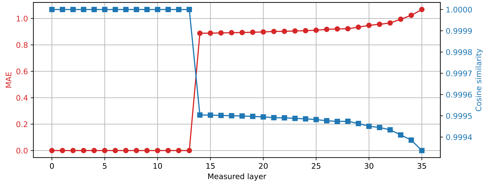
Qwen2.5-3B | Prompt 2 Spared layer 13 | Hybrid vs quantized
