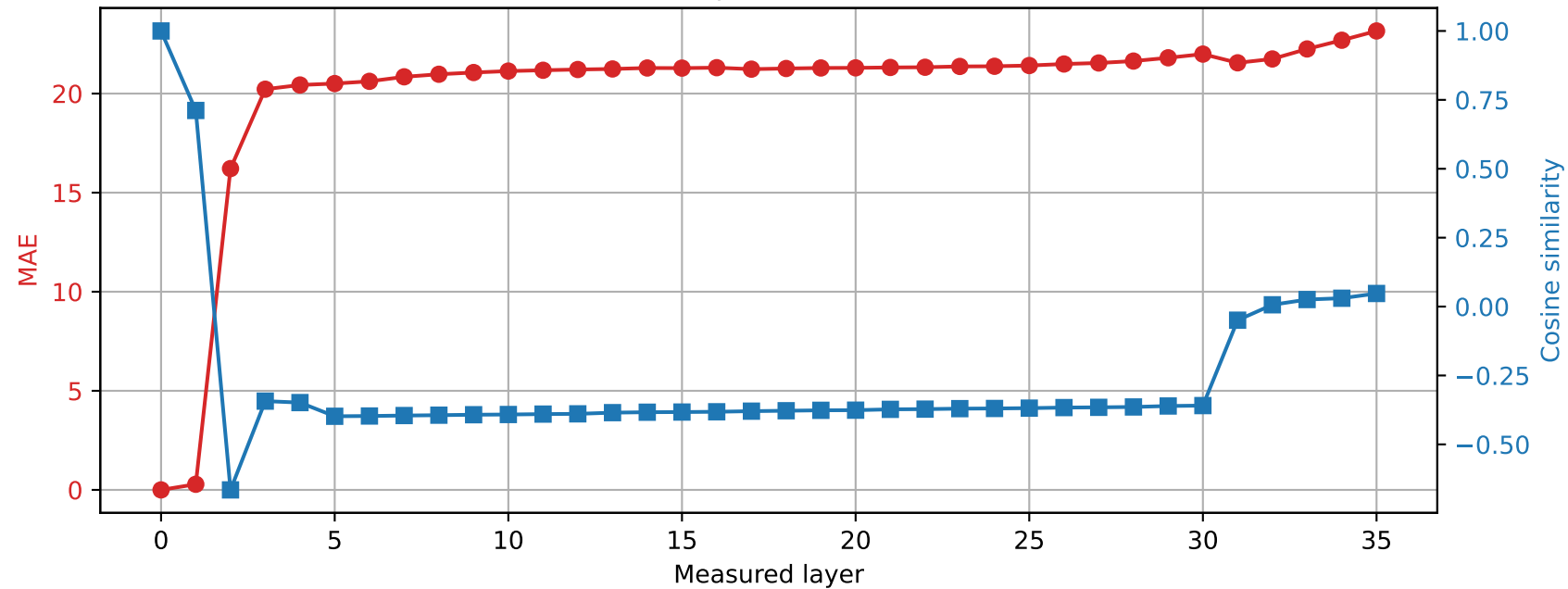
Qwen2.5-3B | Prompt 2 Spared layer 16 | Hybrid vs unquantized
