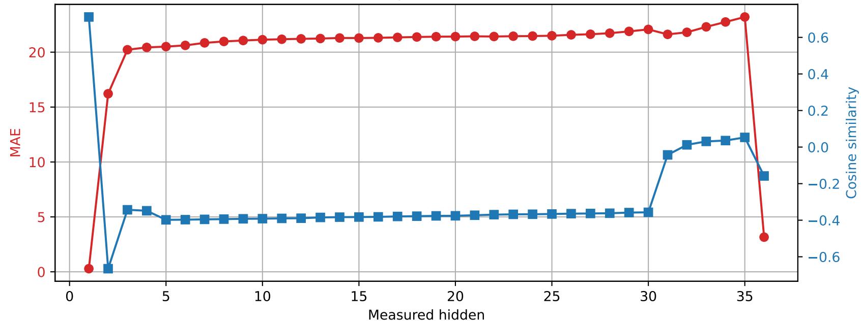
Qwen2.5-3B | Prompt 2 Spared layer 21 | Unquantized vs hybrid
