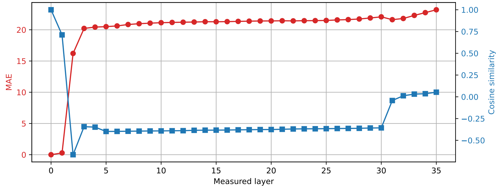
Qwen2.5-3B | Prompt 2 Spared layer 21 | Hybrid vs unquantized
