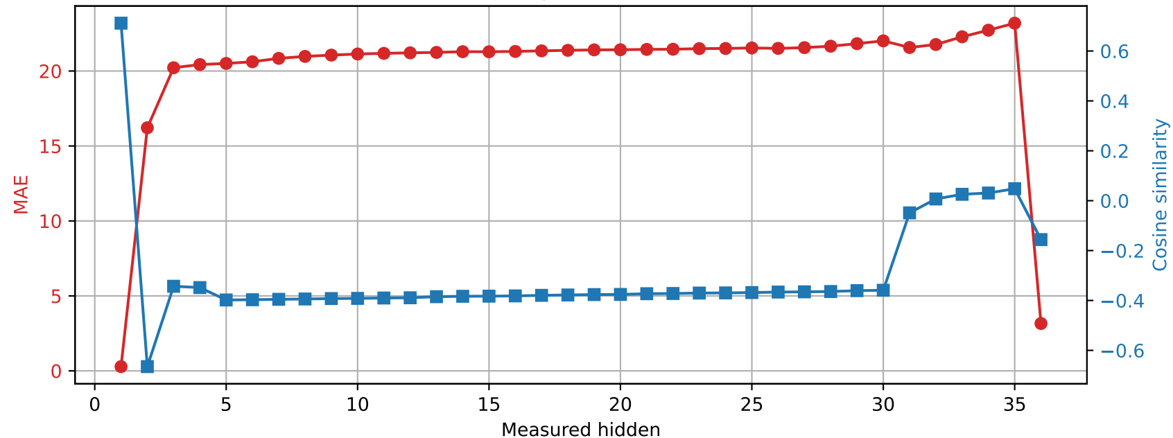
Qwen2.5-3B | Prompt 2 Spared layer 25 | Unquantized vs hybrid
