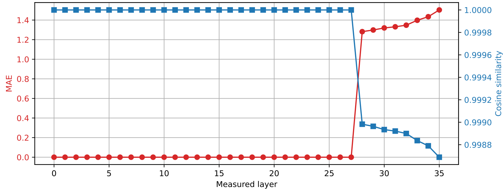
Qwen2.5-3B | Prompt 2 Spared layer 27 | Hybrid vs quantized
