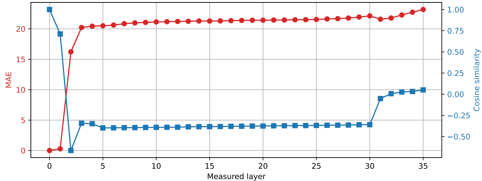
Qwen2.5-3B | Prompt 2 Spared layer 30 | Hybrid vs unquantized
