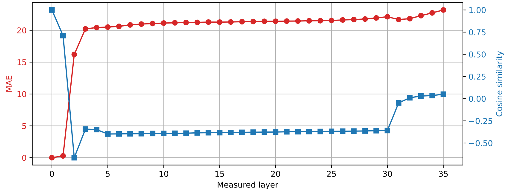
Qwen2.5-3B | Prompt 2 Spared layer 31 | Hybrid vs unquantized
