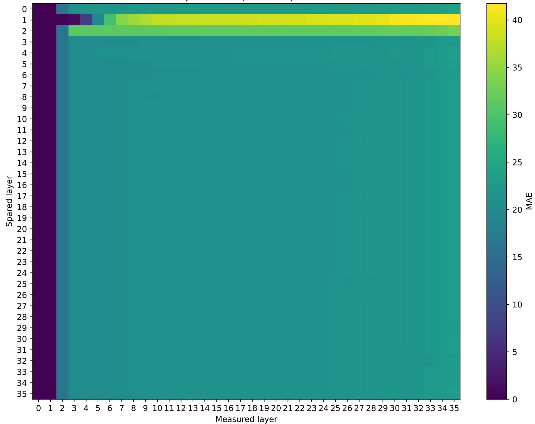
Qwen2.5-3B | Prompt 2 Hybrid vs unquantized | int4
