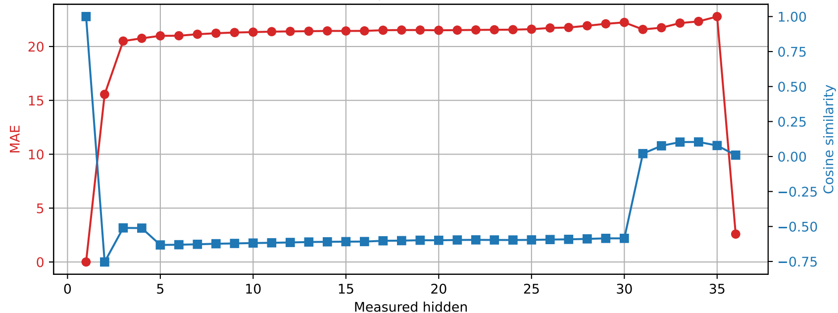
Qwen2.5-3B | Prompt 3 Spared layer 0 | Unquantized vs hybrid
