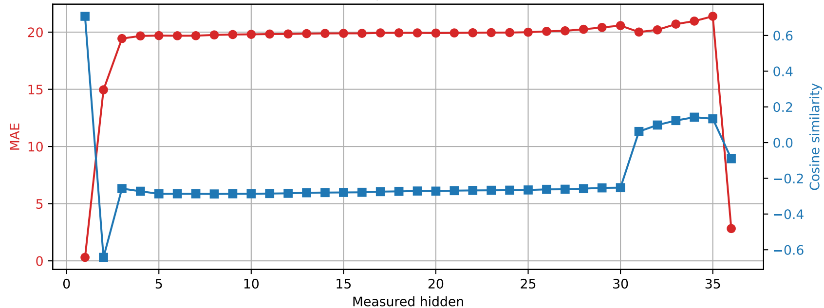
Qwen2.5-3B | Prompt 3 Spared layer 3 | Unquantized vs hybrid
