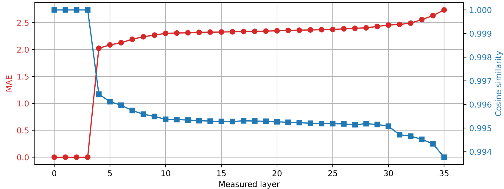
Qwen2.5-3B | Prompt 3 Spared layer 3 | Hybrid vs quantized
