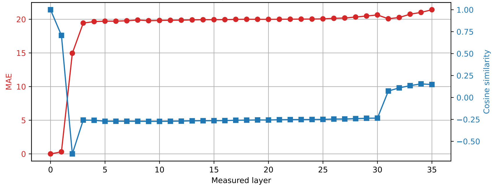
Qwen2.5-3B | Prompt 3 Spared layer 8 | Hybrid vs unquantized
